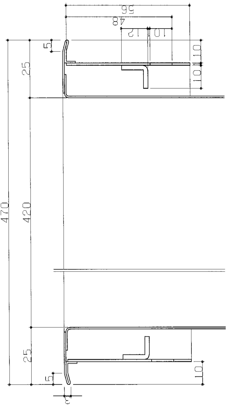
AA断面(1/1)
